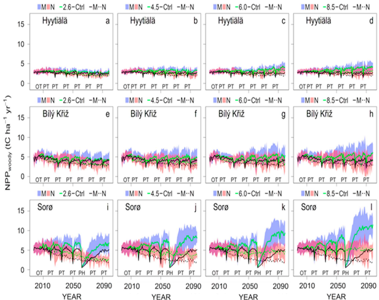
Figure 7. Time series of mean annual NPP wood over the simulation period. Blue shaded area represents the maximum and minimum values for among ESMs and RCPs when management is considered (M), and red shaded area when management is not considered (N). Solid lines represent the average annual values among ESMs for each control (Ctrl) and RCP scenario when management is simulated, and dashed lines when management is not simulated (OT = observed thinning, PT = prescribed thinning, PH = prescribed harvesting). (a, e, and i) Simulations under RCP2.6 scenario; (b, f, j) RCP4.5 scenario; (c, g, k) RCP6.0 scenario; and (d, h, l) RCP8.5 scenario. ESMs = Earth System Models; RCPs = Representative Concentration Pathways; NPP = net primary production.
