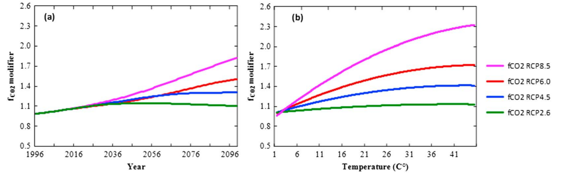
Figure 1. Trends for the f_{CO_2} modifier for assimilation based on the climate change using four Representative Concentration Pathways (RCPs 2.6, 4.5, 6.0, 8.5) used for forcing the model (reference [CO_2] \sim 370 ppmv): (a) variations of modifier related to changes of [CO_2] along the simulation period at fixed temperature 20 °C; (b) sensitivity of f_{CO_2} modifier at fixed [CO_2] (based on the 2099 values for each RCPs) and variable temperature. Parameterization for equations (1)–(4) follows from values given in Veroustraete (1994) and Veroustraete et al. (2002).
